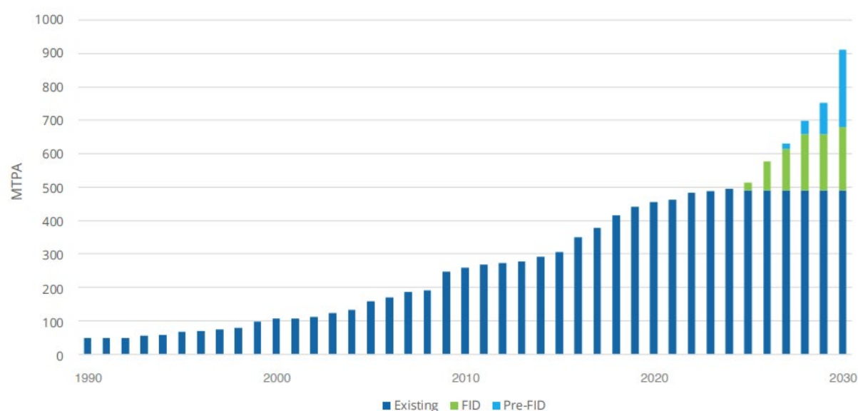
Figure 5.4: Global liquefaction capacity development, 1990-2030
